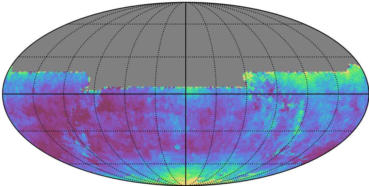
weather_cloudso20v3.4_10yrs All sky y band: Median seeingEff
