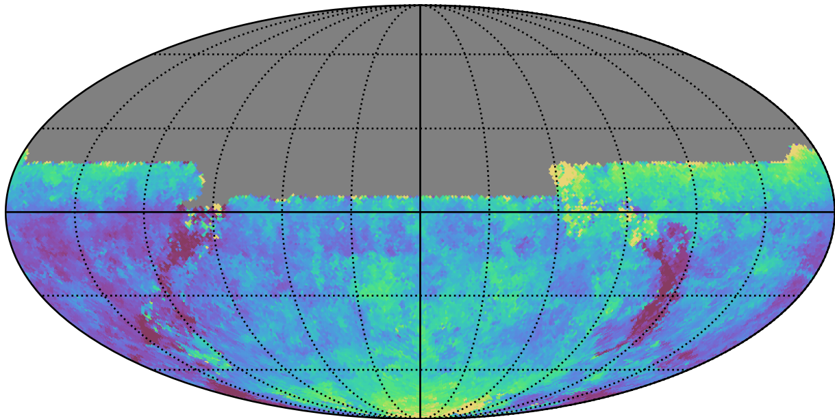
weather_cloudso20v3.4_10yrs All sky u band: Median seeingEff
