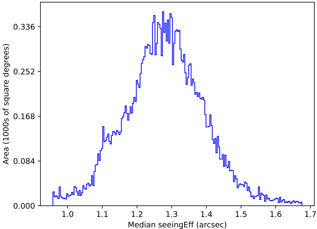
weather_cloudso20v3.4_10yrs All sky u band: Median seeingEff
