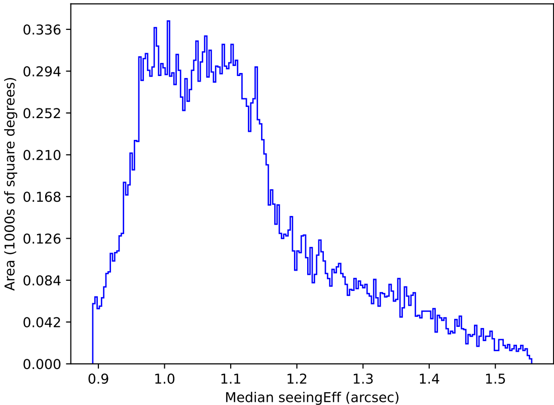
weather_cloudso20v3.4_10yrs All sky r band: Median seeingEff
