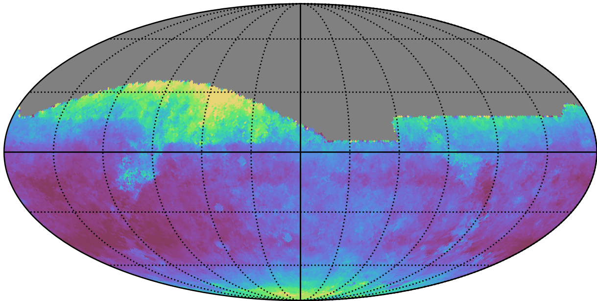
weather_cloudso20v3.4_10yrs All sky i band: Median seeingEff
