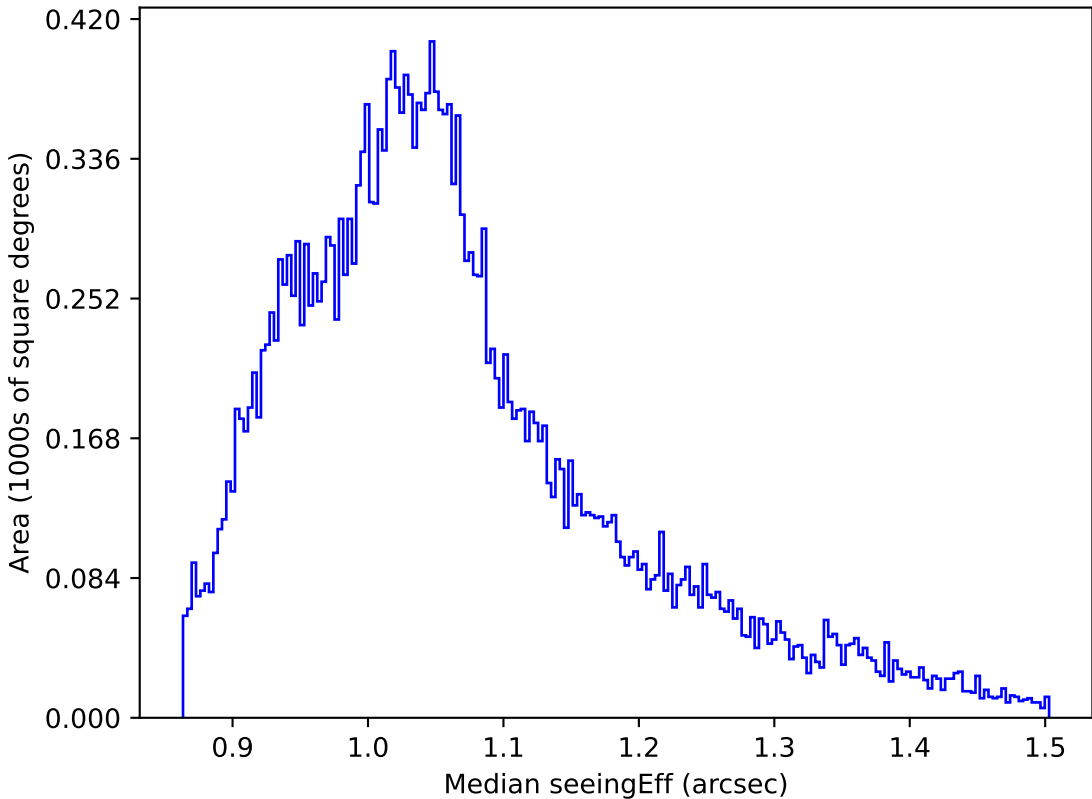
weather_cloudso20v3.4_10yrs All sky i band: Median seeingEff
