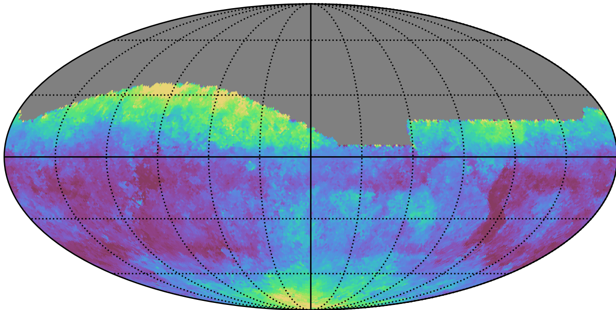
weather_cloudso20v3.4_10yrs All sky g band: Median seeingEff
