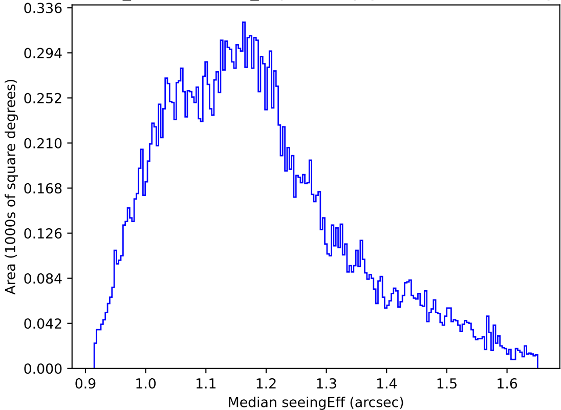
weather_cloudso20v3.4_10yrs All sky g band: Median seeingEff
