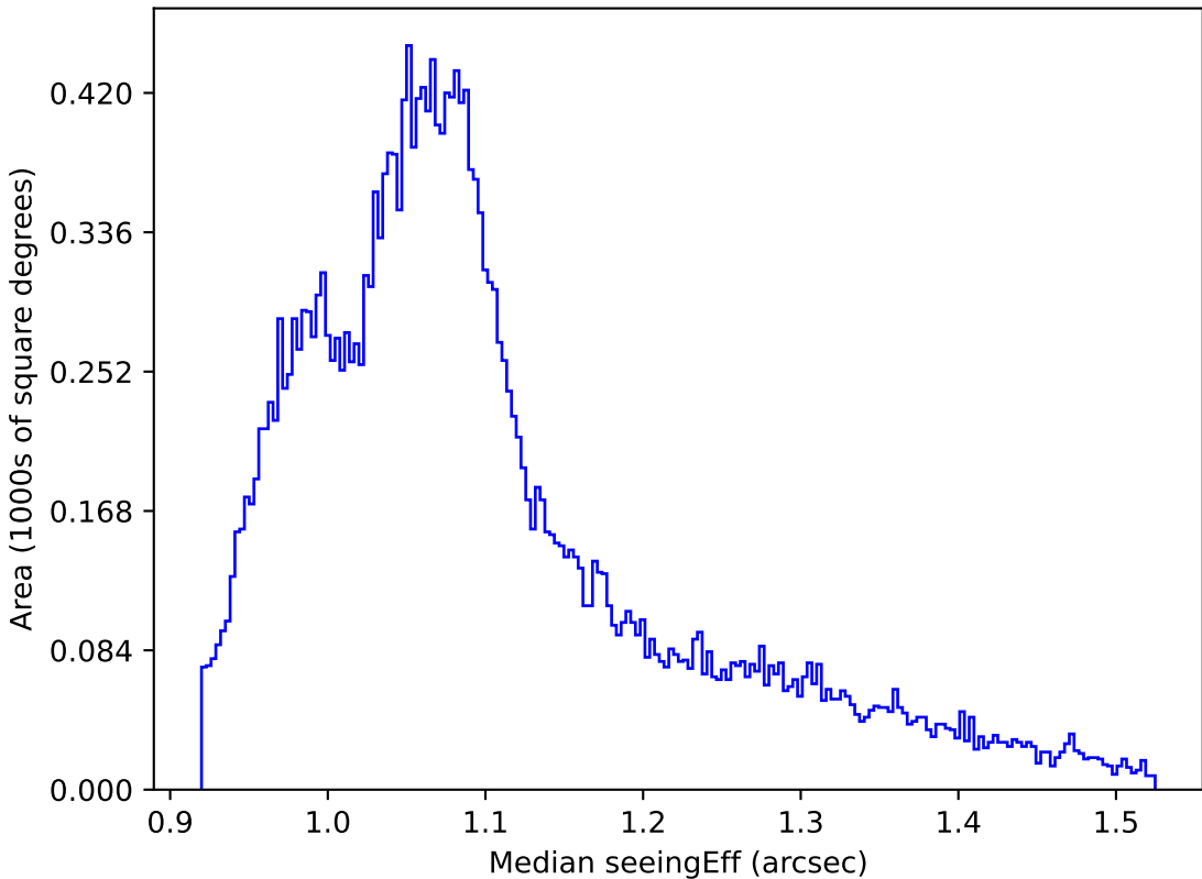
weather_cloudso20v3.4_10yrs All sky all bands: Median seeingEff
