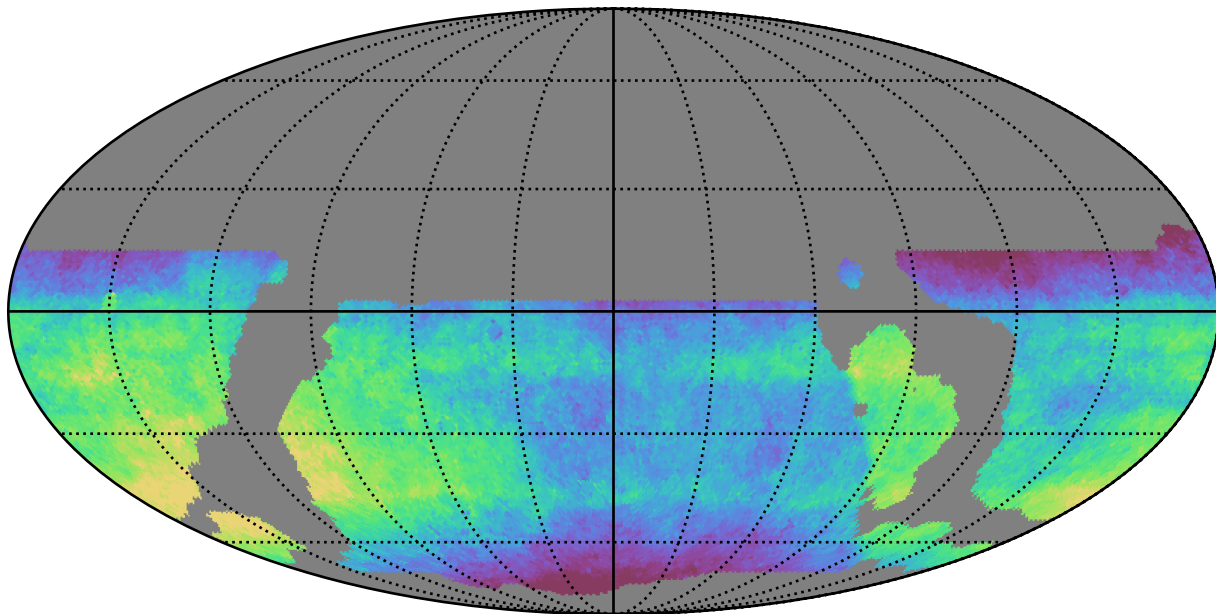
weather_cloudso20v3.4_10yrs WFD all bands: Median saturation_mag
