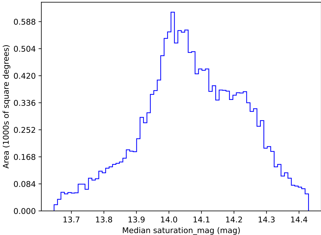
weather_cloudso20v3.4_10yrs WFD all bands: Median saturation_mag
