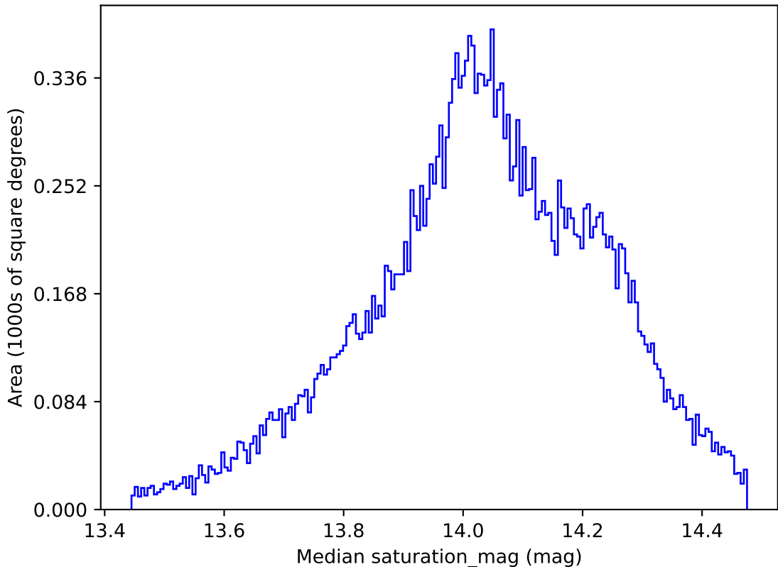
weather_cloudso20v3.4_10yrs All sky all bands: Median saturation_mag
