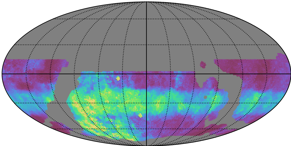
weather_cloudso20v3.4_10yrs WFD u band: Median normairmass
