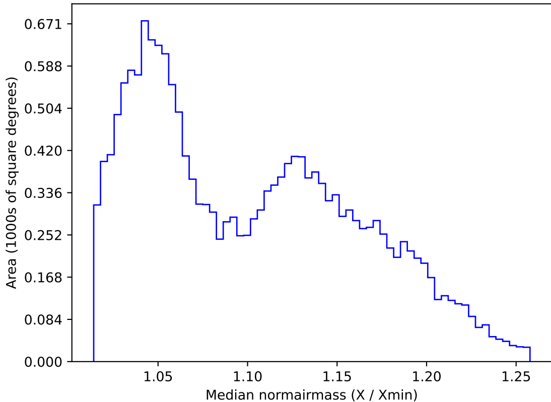
weather_cloudso20v3.4_10yrs WFD u band: Median normairmass
