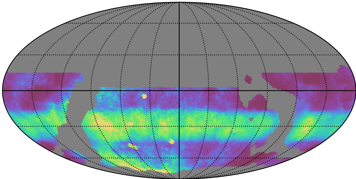
weather_cloudso20v3.4_10yrs WFD r band: Median normairmass
