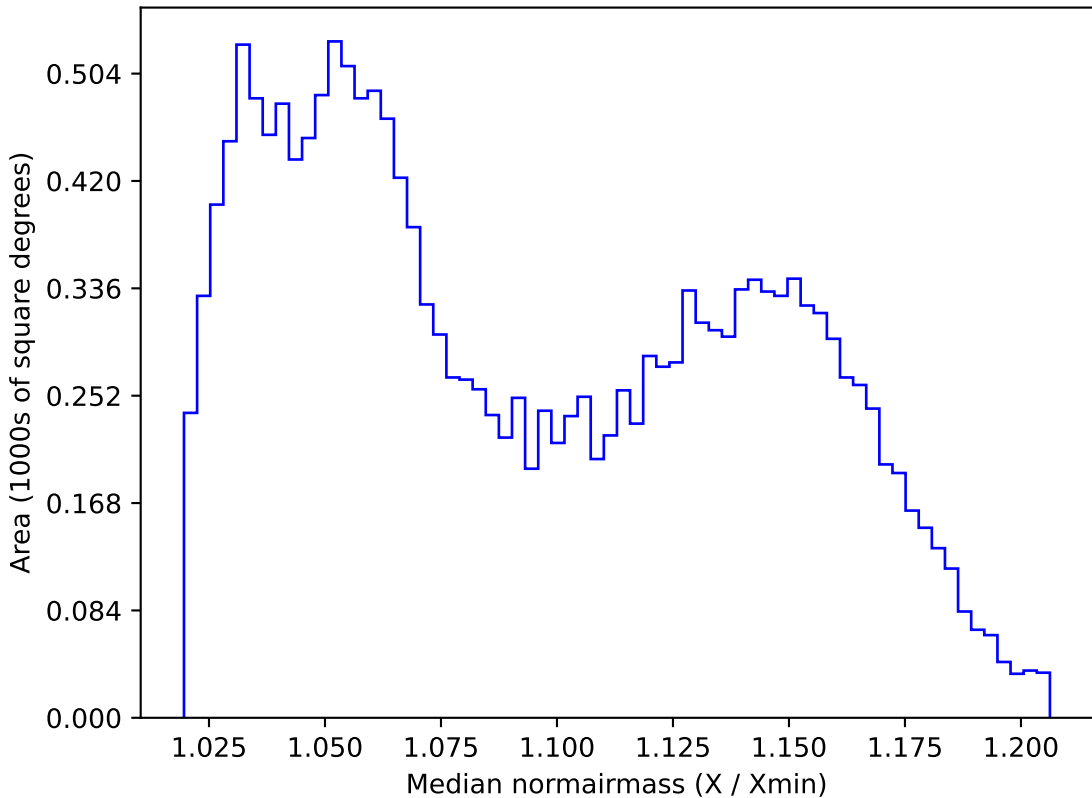
weather_cloudso20v3.4_10yrs WFD r band: Median normairmass
