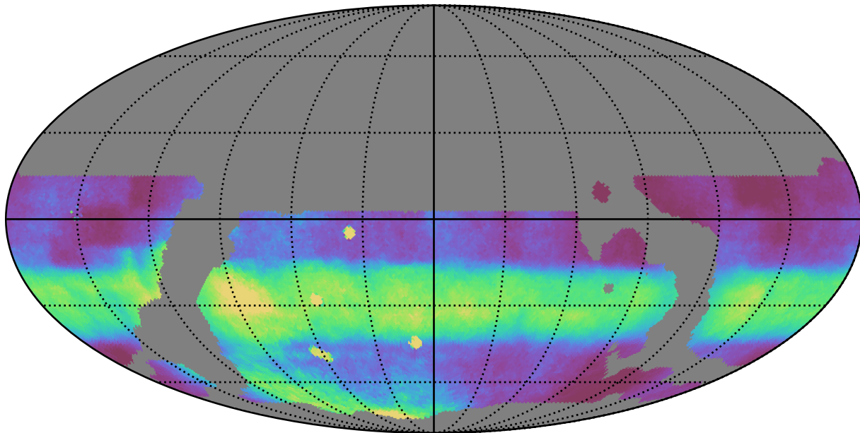
weather_cloudso20v3.4_10yrs WFD all bands: Median normairmass
