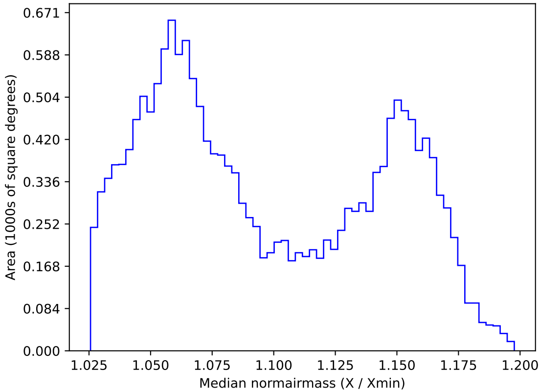
weather_cloudso20v3.4_10yrs WFD all bands: Median normairmass
