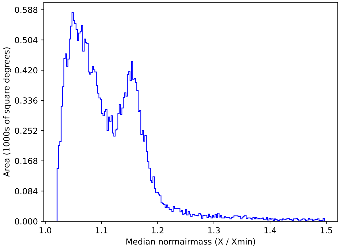
weather_cloudso20v3.4_10yrs All sky z band: Median normairmass
