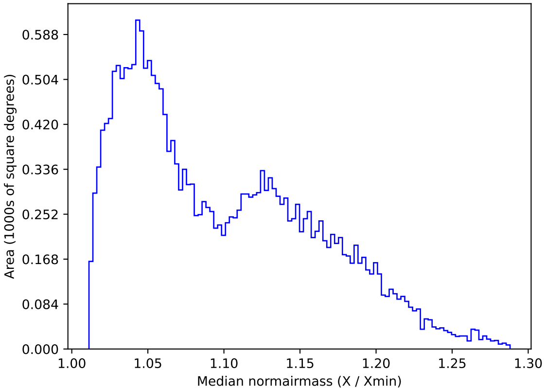
weather_cloudso20v3.4_10yrs All sky u band: Median normairmass
