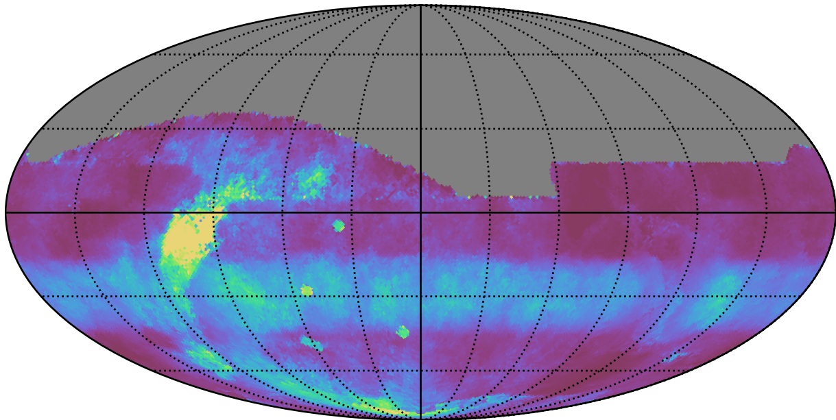
weather_cloudso20v3.4_10yrs All sky r band: Median normairmass
