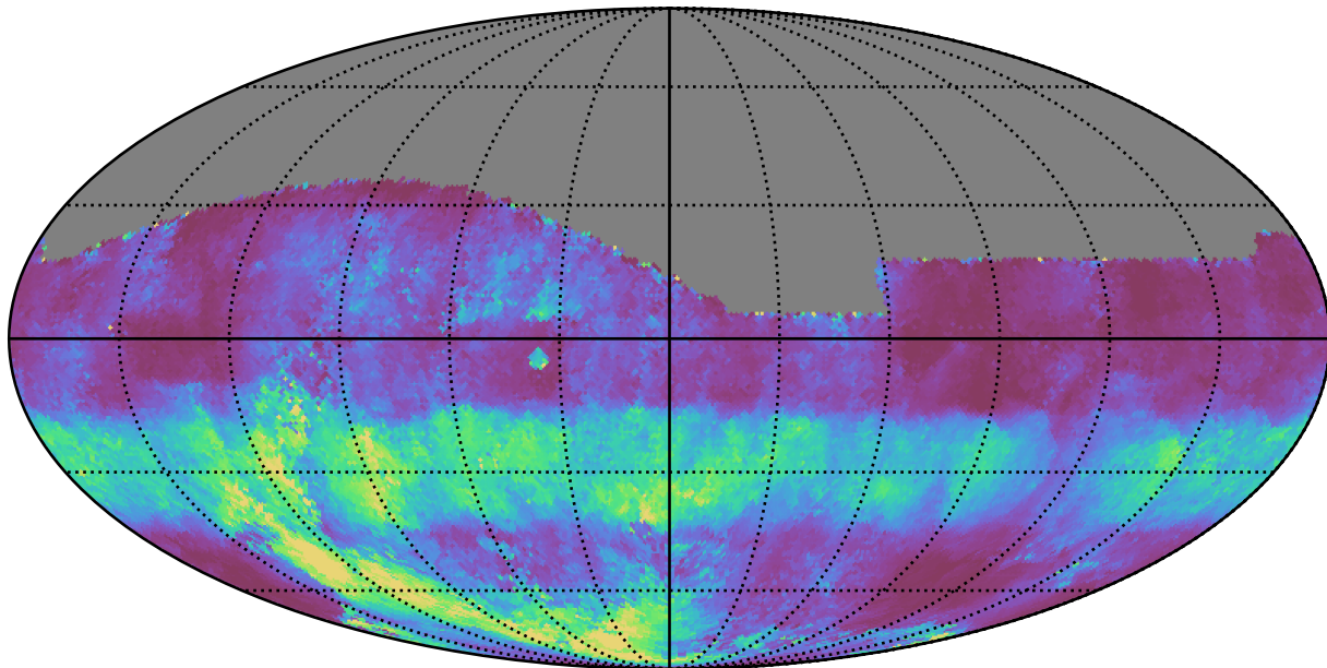
weather_cloudso20v3.4_10yrs All sky g band: Median normairmass
