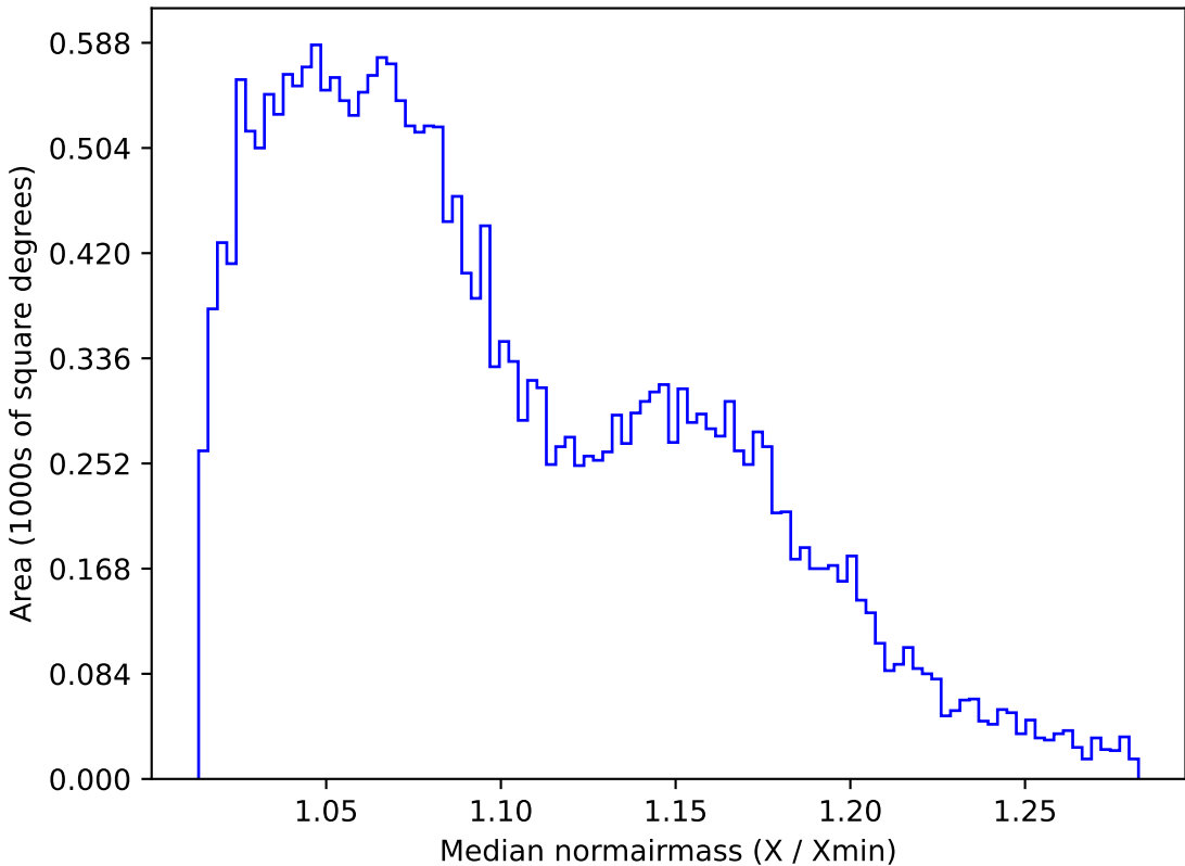
weather_cloudso20v3.4_10yrs All sky g band: Median normairmass
