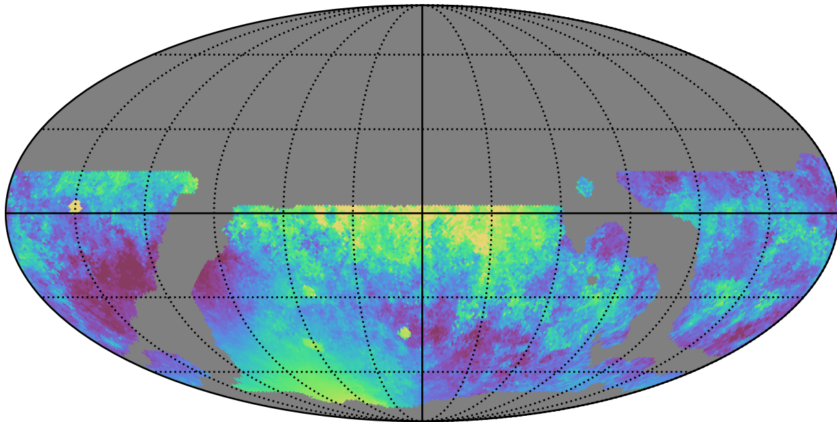
weather_cloudso20v3.4_10yrs WFD z band: Median moonDistance
