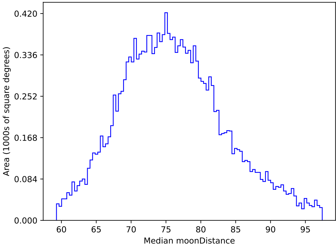
weather_cloudso20v3.4_10yrs WFD z band: Median moonDistance
