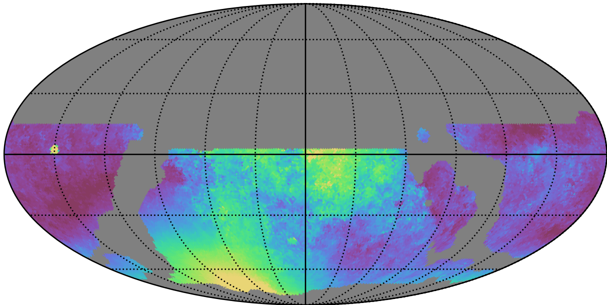
weather_cloudso20v3.4_10yrs WFD y band: Median moonDistance
