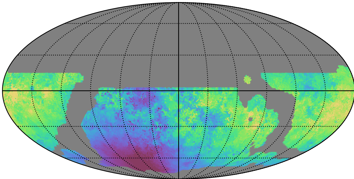
weather_cloudso20v3.4_10yrs WFD u band: Median moonDistance
