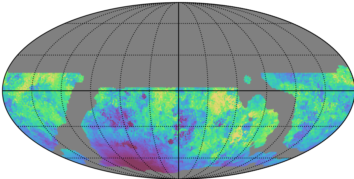
weather_cloudso20v3.4_10yrs WFD g band: Median moonDistance
