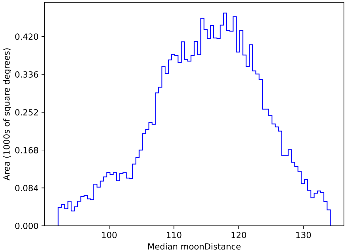
weather_cloudso20v3.4_10yrs WFD g band: Median moonDistance
