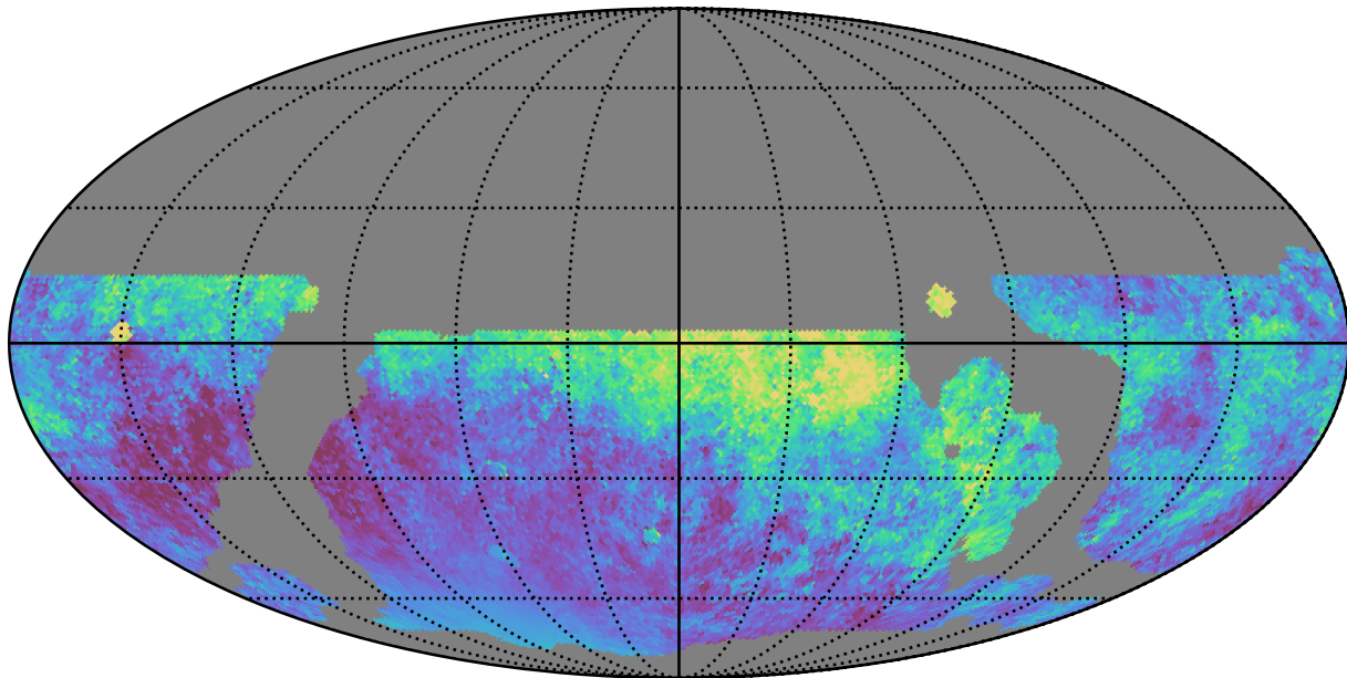
weather_cloudso20v3.4_10yrs WFD all bands: Median moonDistance
