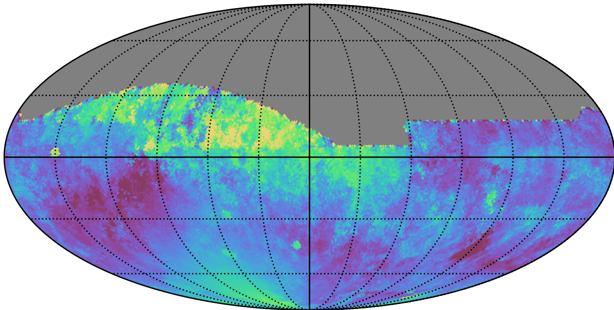
weather_cloudso20v3.4_10yrs All sky z band: Median moonDistance
