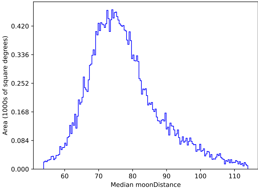
weather_cloudso20v3.4_10yrs All sky z band: Median moonDistance
