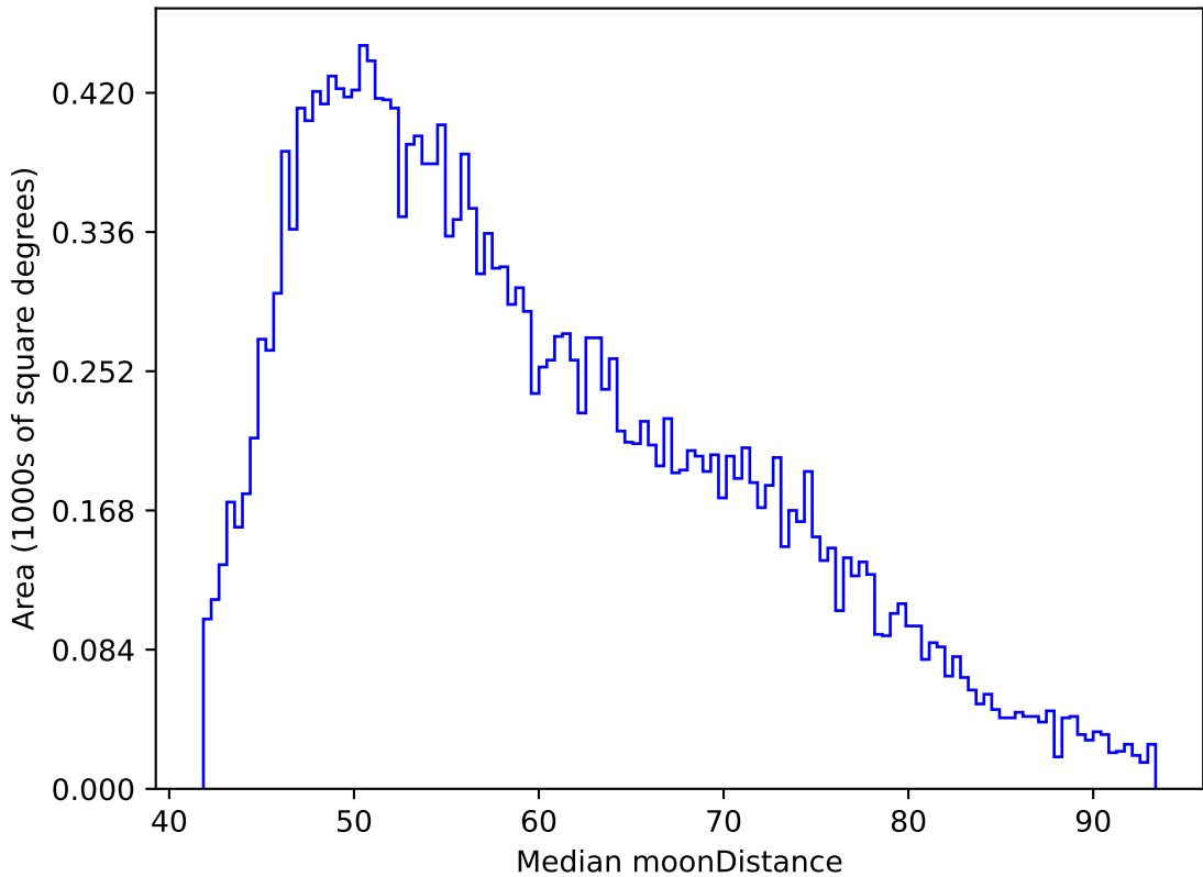
weather_cloudso20v3.4_10yrs All sky y band: Median moonDistance
