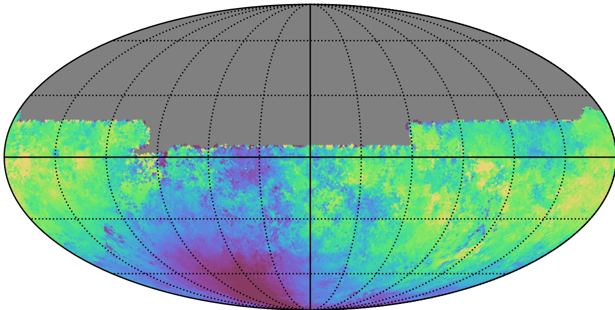
weather_cloudso20v3.4_10yrs All sky u band: Median moonDistance
