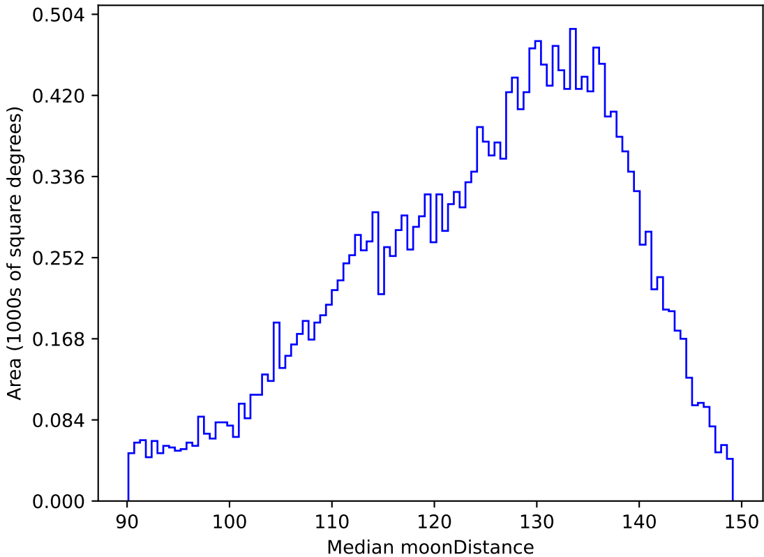
weather_cloudso20v3.4_10yrs All sky u band: Median moonDistance
