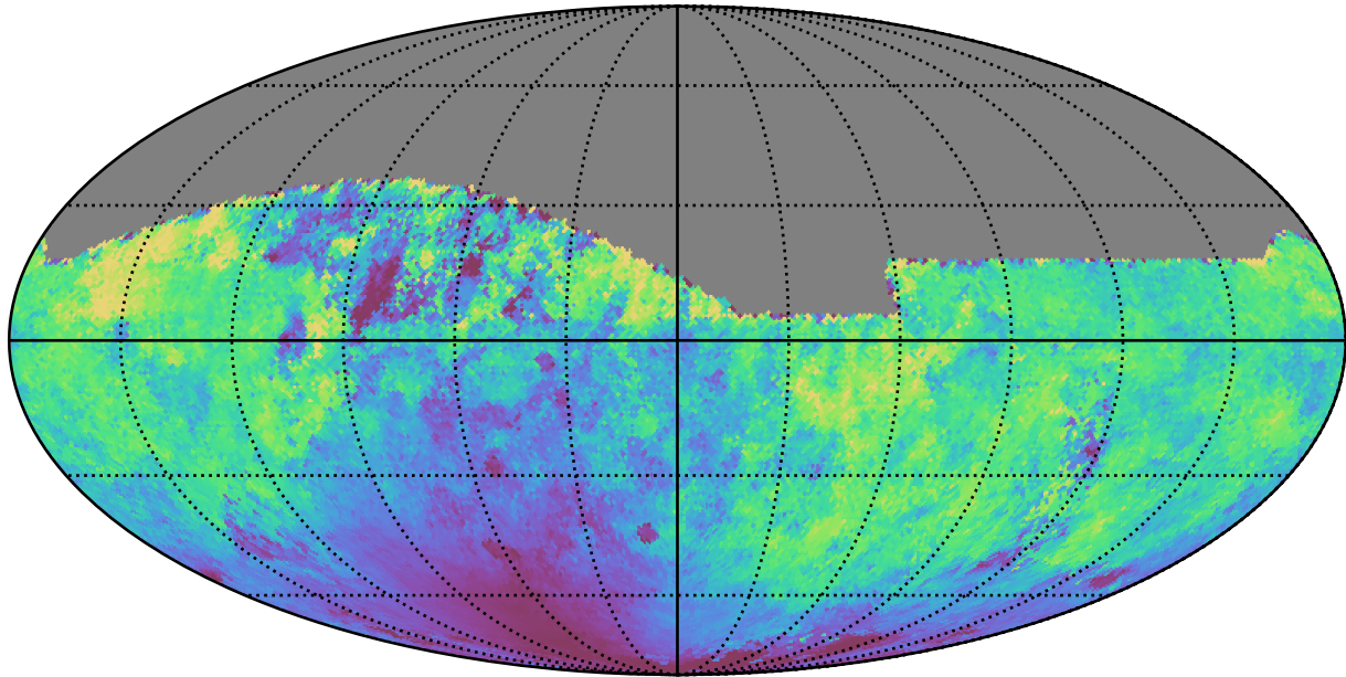
weather_cloudso20v3.4_10yrs All sky r band: Median moonDistance
