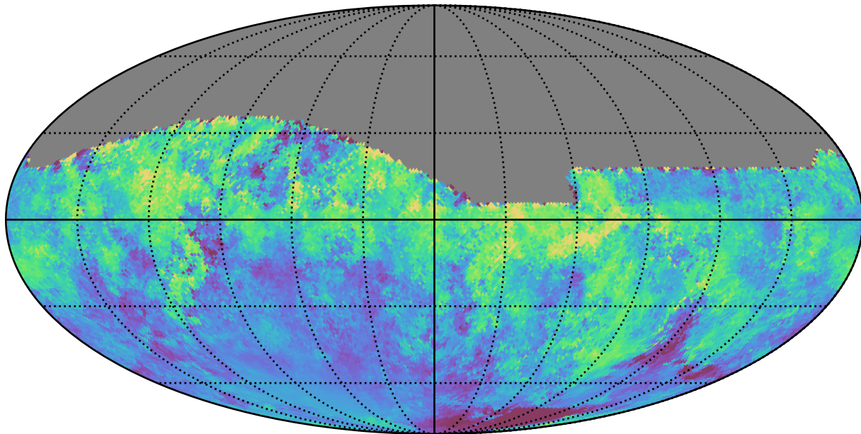
weather_cloudso20v3.4_10yrs All sky i band: Median moonDistance
