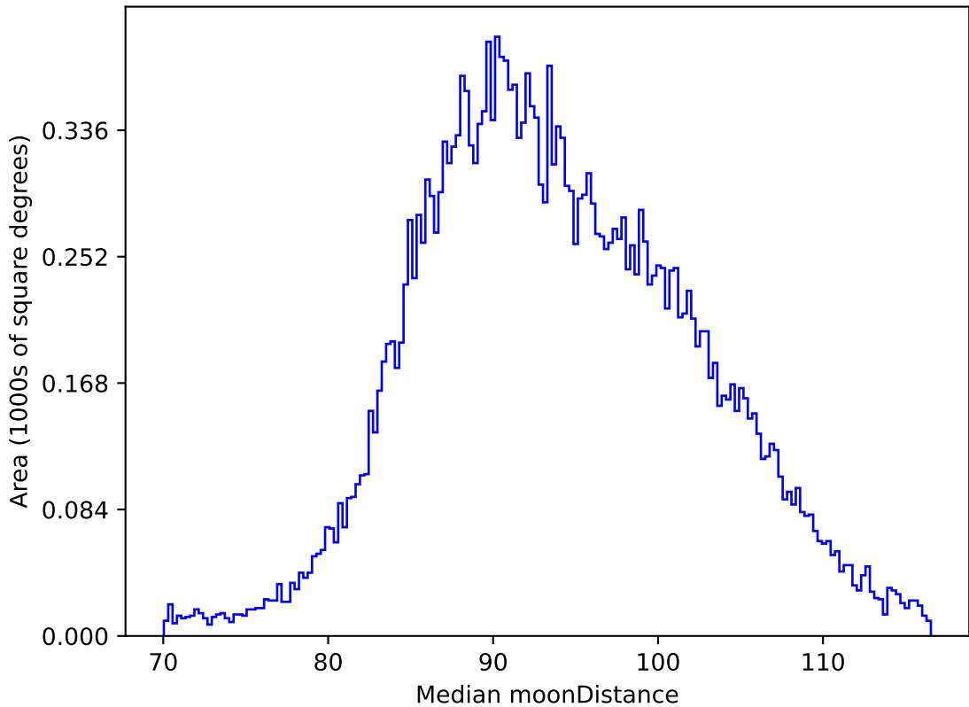
weather_cloudso20v3.4_10yrs All sky i band: Median moonDistance
