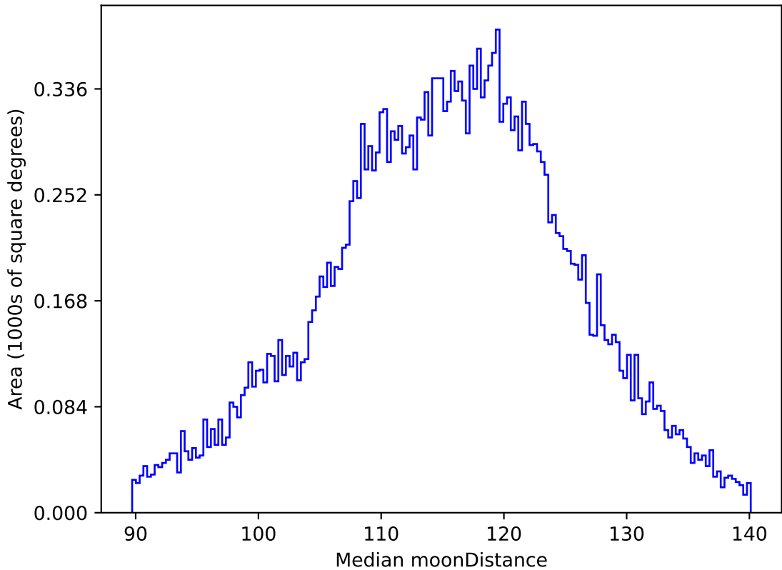
weather_cloudso20v3.4_10yrs All sky g band: Median moonDistance
