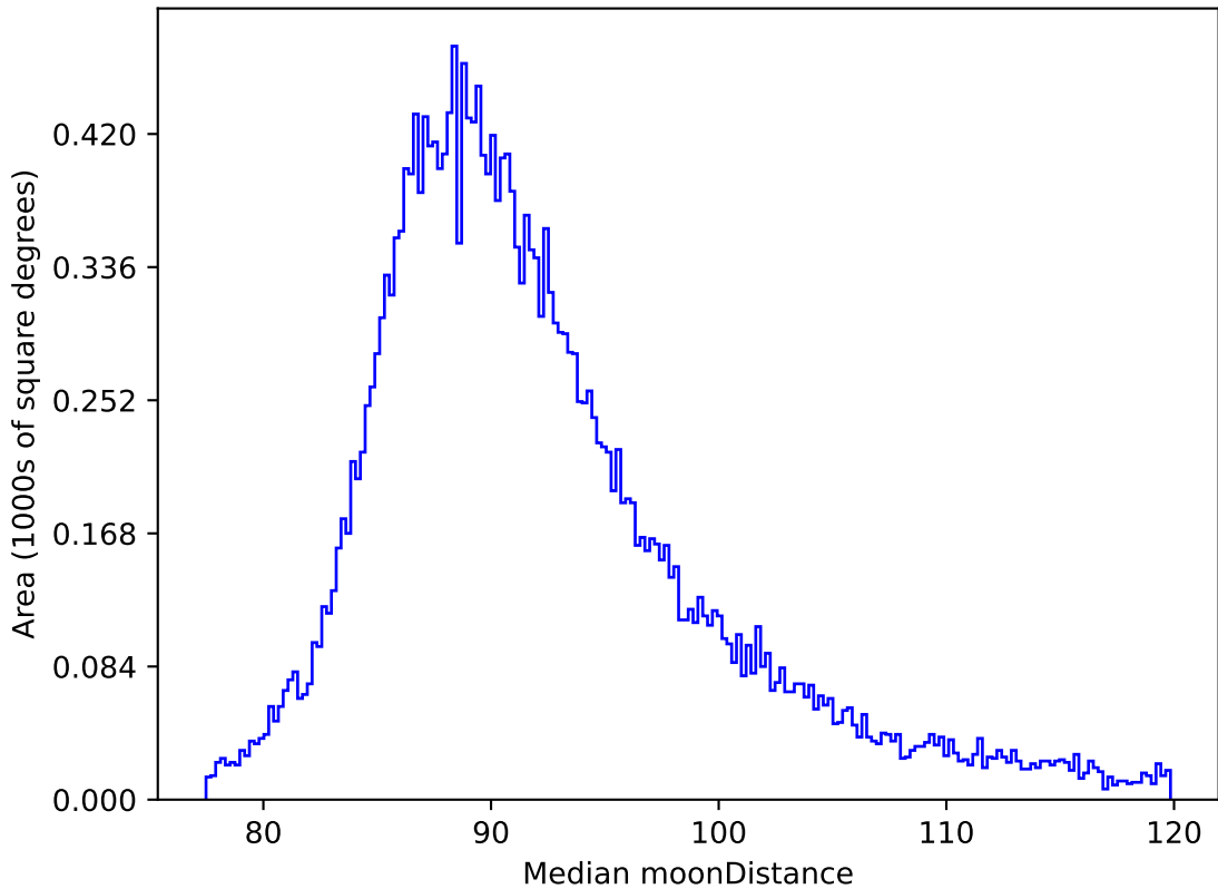
weather_cloudso20v3.4_10yrs All sky all bands: Median moonDistance
