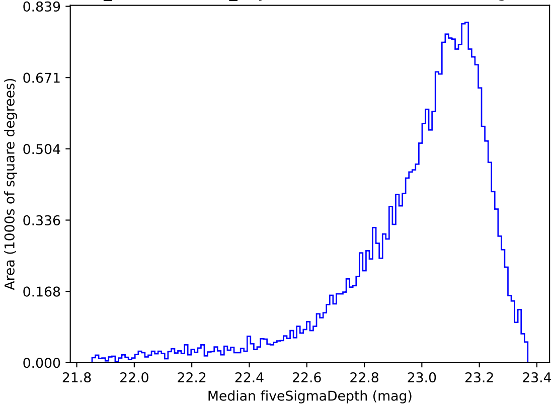
weather_cloudso20v3.4_10yrs Yr 1 z band: Median fiveSigmaDepth
