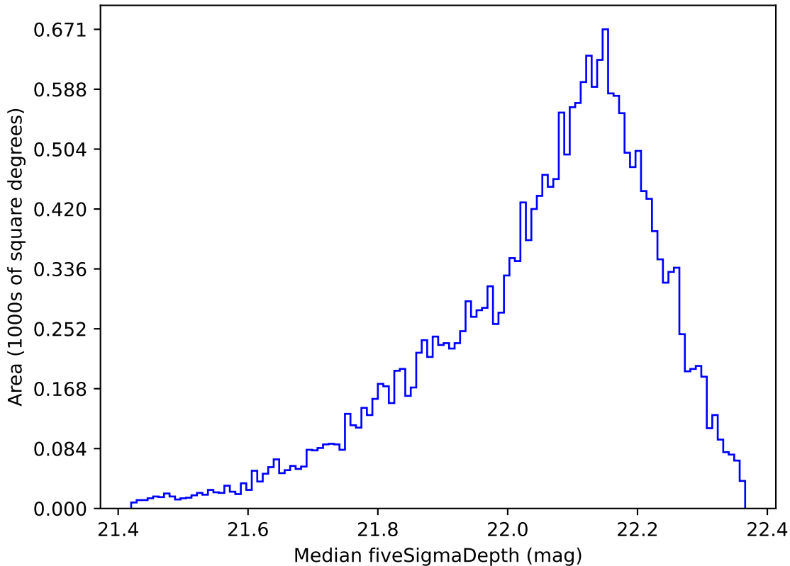
weather_cloudso20v3.4_10yrs Yr 1 y band: Median fiveSigmaDepth
