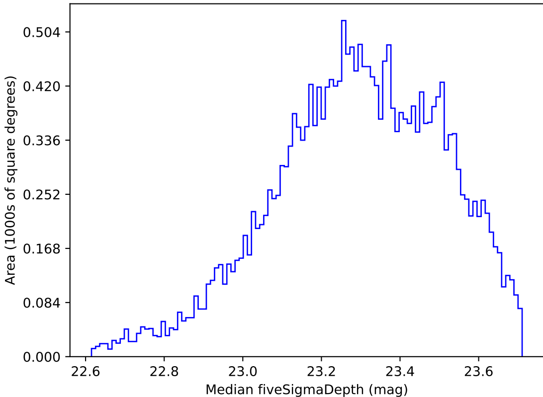
weather_cloudso20v3.4_10yrs Yr 1 u band: Median fiveSigmaDepth
