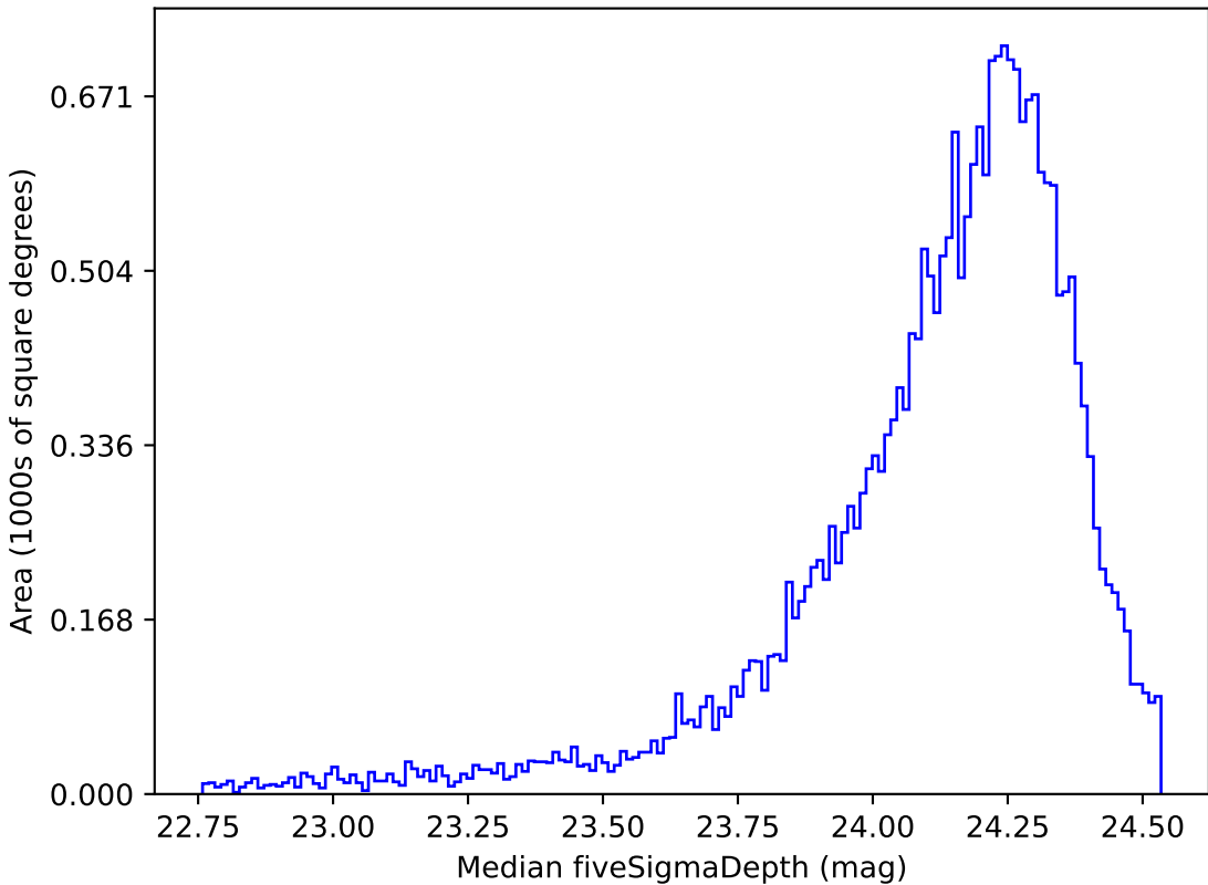
weather_cloudso20v3.4_10yrs Yr 1 r band: Median fiveSigmaDepth
