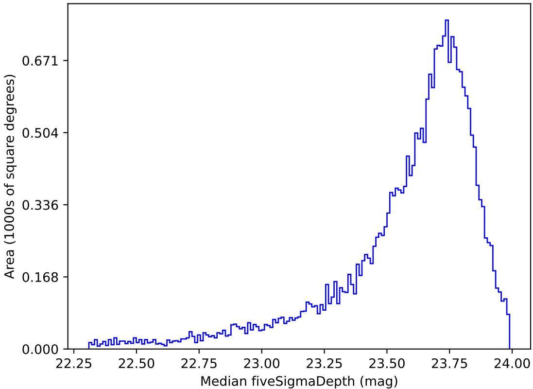
weather_cloudso20v3.4_10yrs Yr 1 i band: Median fiveSigmaDepth
