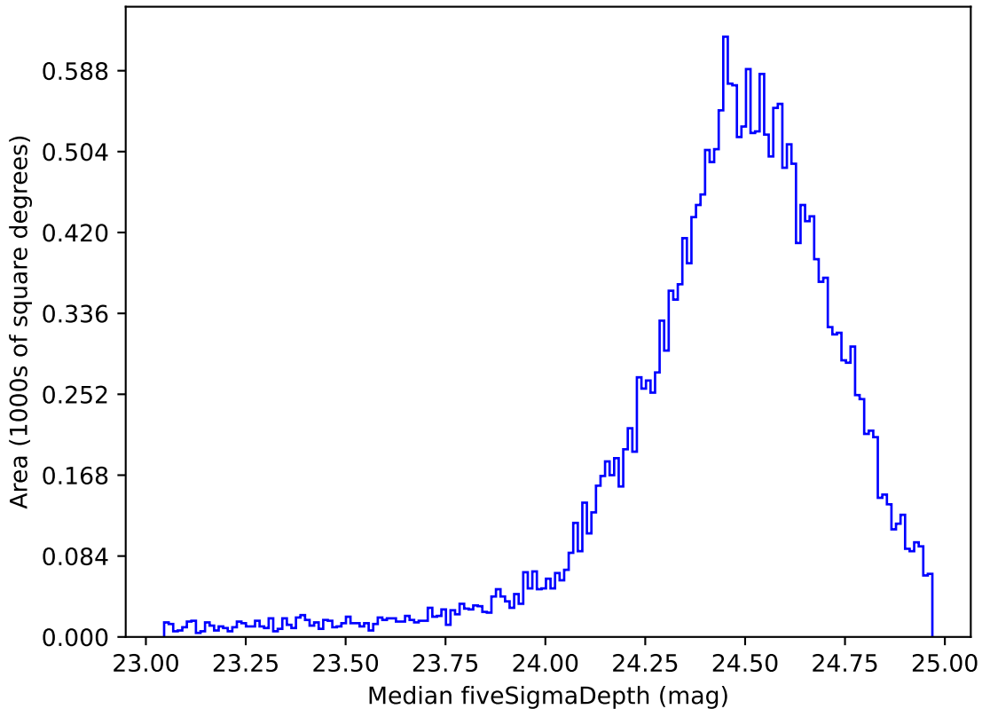
weather_cloudso20v3.4_10yrs Yr 1 g band: Median fiveSigmaDepth
