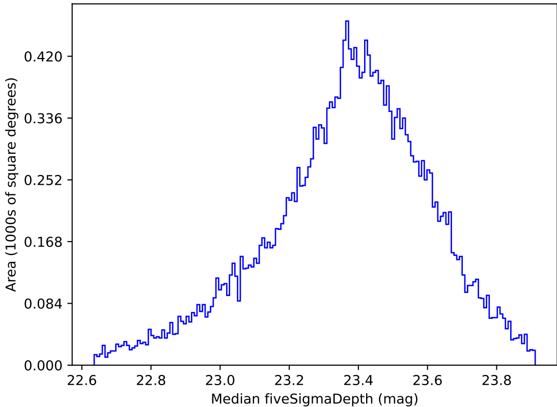
weather_cloudso20v3.4_10yrs Yr 1 all bands: Median fiveSigmaDepth
