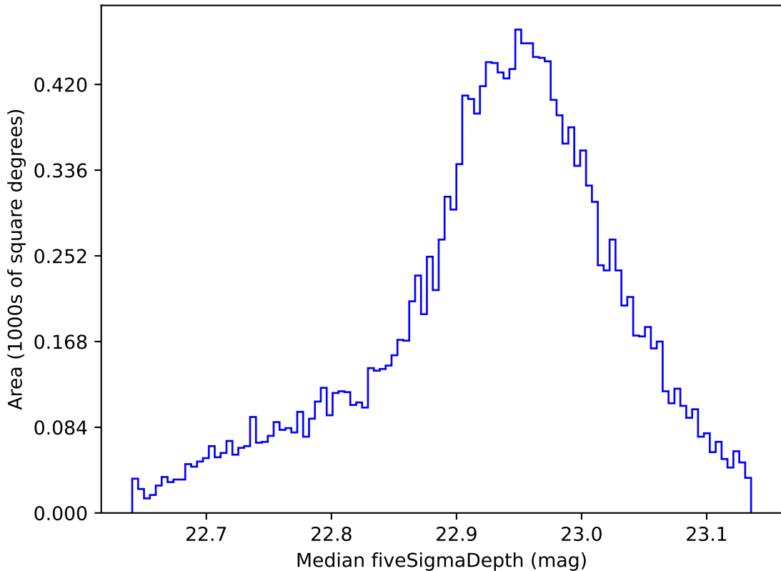
weather_cloudso20v3.4_10yrs WFD z band: Median fiveSigmaDepth
