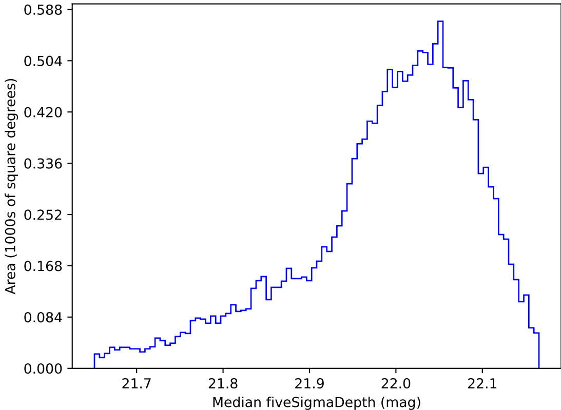
weather_cloudso20v3.4_10yrs WFD y band: Median fiveSigmaDepth
