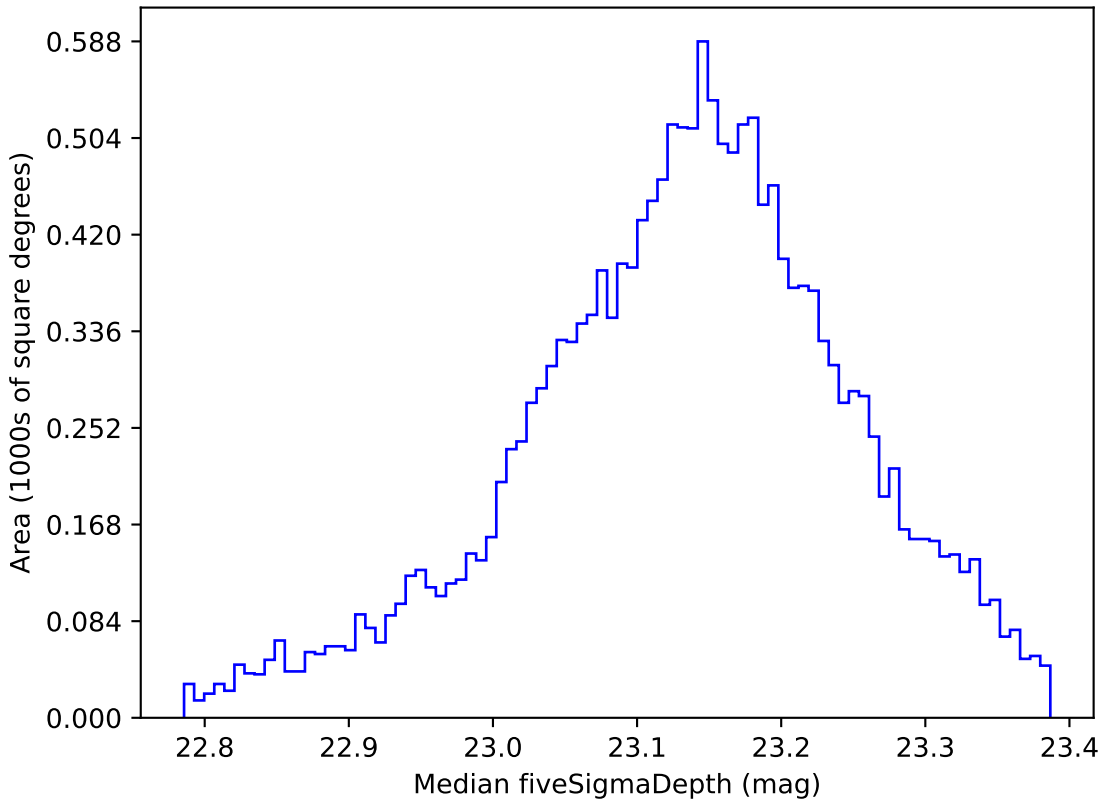
weather_cloudso20v3.4_10yrs WFD u band: Median fiveSigmaDepth
